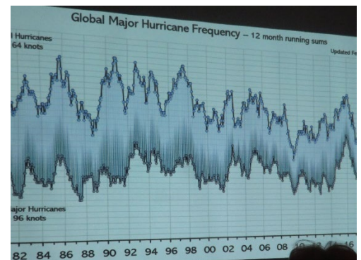
Chart of Major Hurricane Frequency
