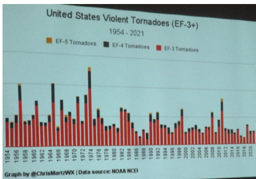
Chart of Violent Tornadoes
